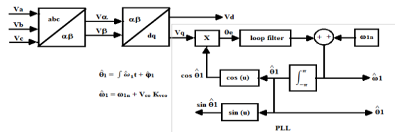
Figure 6: Secondary control technique
