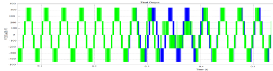
Figure 13: Response of grid voltage and DG voltage during voltage sags in Droop control technique
