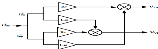
Figure 4: Fundamental virtual impedance loop
