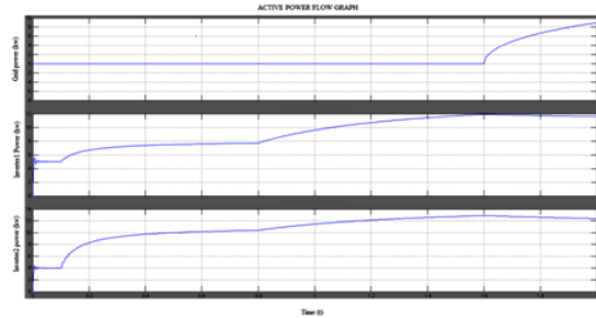
Figure 16: Power sharing graph
