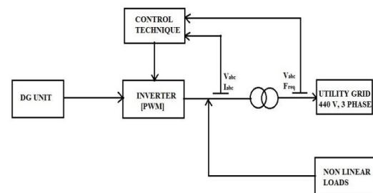
Figure 2: Block Diagram of Droop Control
