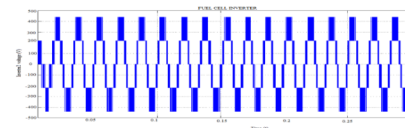
Figure 11: voltage waveform of fuel cell inverter
