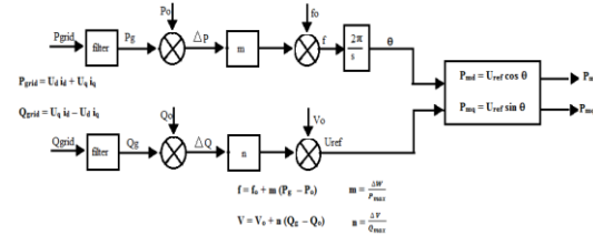
Figure 5: Primary control technique
