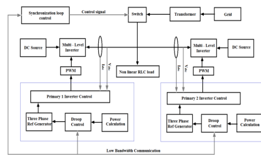
Figure 1: Block diagram of Enhanced droop control system
