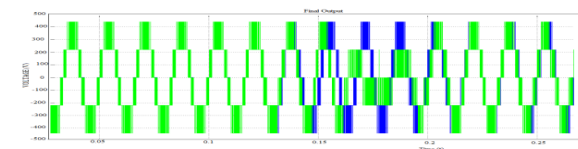
Figure 12: Response of grid voltage and DG voltage when Non - linear load increases in Enhanced Droop control
