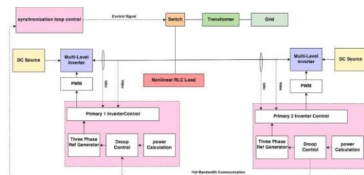
Figure 3: Block Diagram of Decentralized Droop Control
